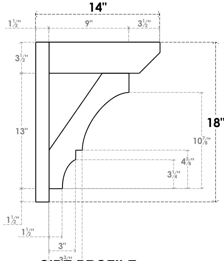
SIDE PROFILE
